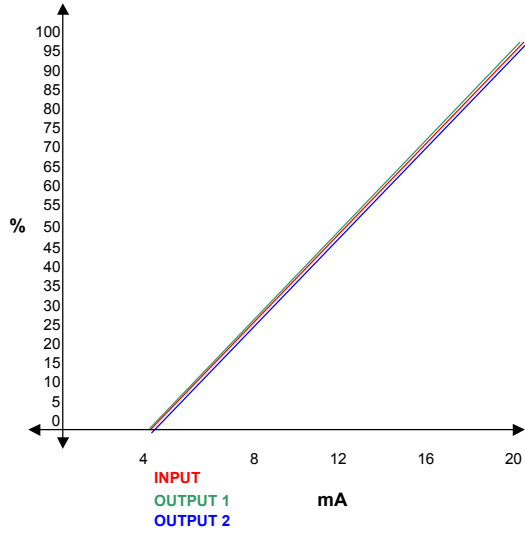
MINIMUM 30/70 SPLITTER
