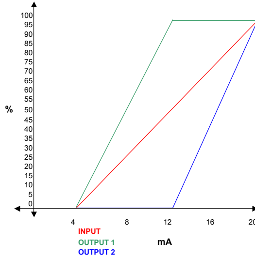
MAXIMUM 70/30 SPLITTER
